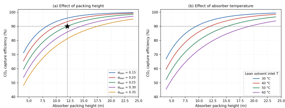
Figure 5: Absorber sensitivity. (a) Capture efficiency versus packing height at five lean loadings; (b) effect of lean solvent inlet temperature
