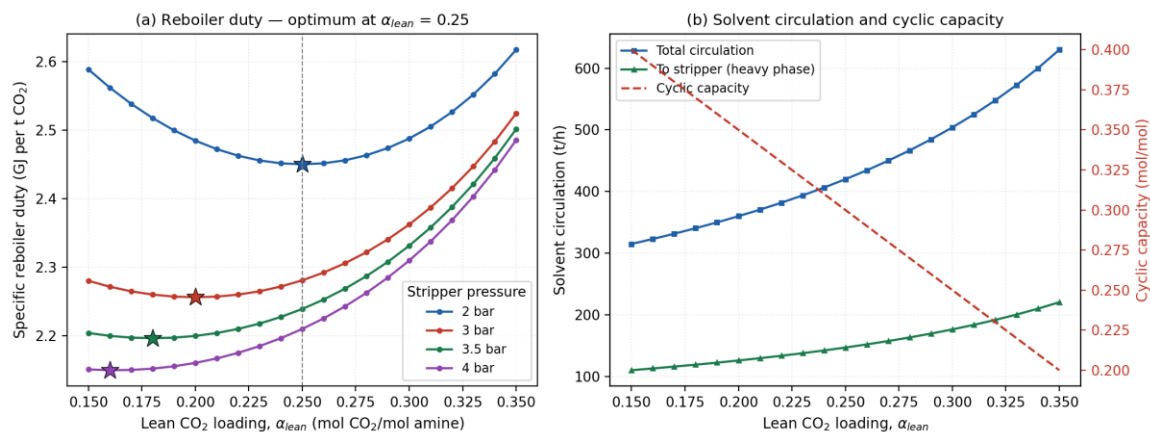
Figure 2: Effect of lean \text{CO}_2 loading. (a) Specific reboiler duty at four stripper pressures, stars indicating the optimum in each case; (b) solvent circulation, circulation to the stripper and cyclic capacity
