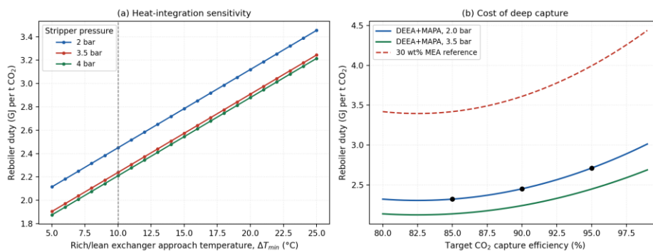
Figure 6: (a) Sensitivity of reboiler duty to the rich/lean exchanger approach temperature at three stripper pressures; (b) reboiler duty versus target capture efficiency, compared with the 30 wt% MEA reference.
