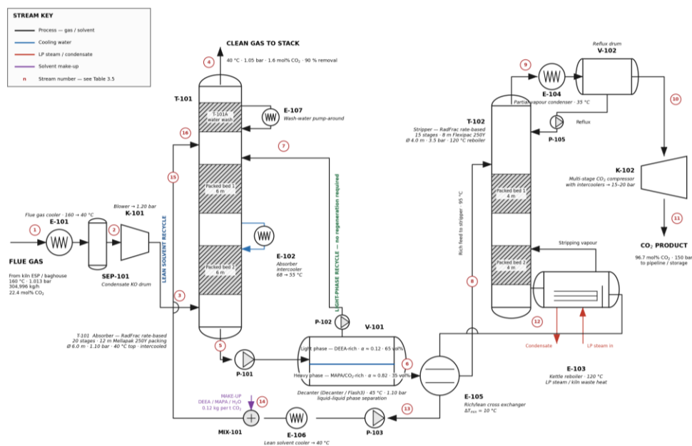
Figure 1. Aspen Plus V14 process flowsheet for CO 2 capture from Ashaka cement kiln flue gas using 5 M DEEA + 2 M MAPA phase-change solvent
