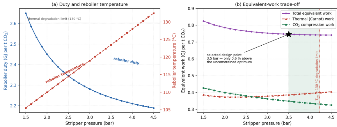
Figure 3. Effect of stripper pressure. (a) Specific reboiler duty and reboiler temperature; (b) decomposition of total equivalent work, with the 130 °C thermal degradation limit indicated
