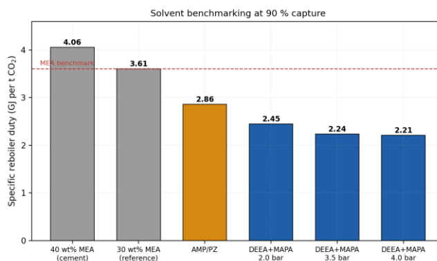
Figure 7. Specific reboiler duty of the DEEA–MAPA blend compared with MEA and AMP/PZ benchmarks at 90 % capture.
