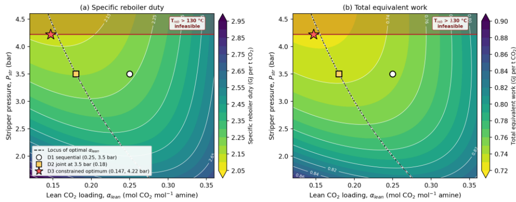
Figure 4. Design surfaces over the coupled lean-loading–pressure space. (a) Specific reboiler duty; (b) total equivalent work. The dashed line is the locus of optimal lean loading, the shaded band the thermally infeasible region, and the markers the three design points of Table 5
